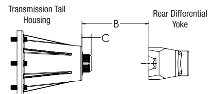
Detailed View Minus the Driveshaft
